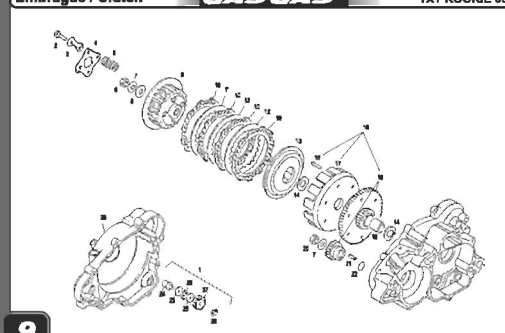
Embrague / Clutch GASGAS TXT ROOKIE 05
