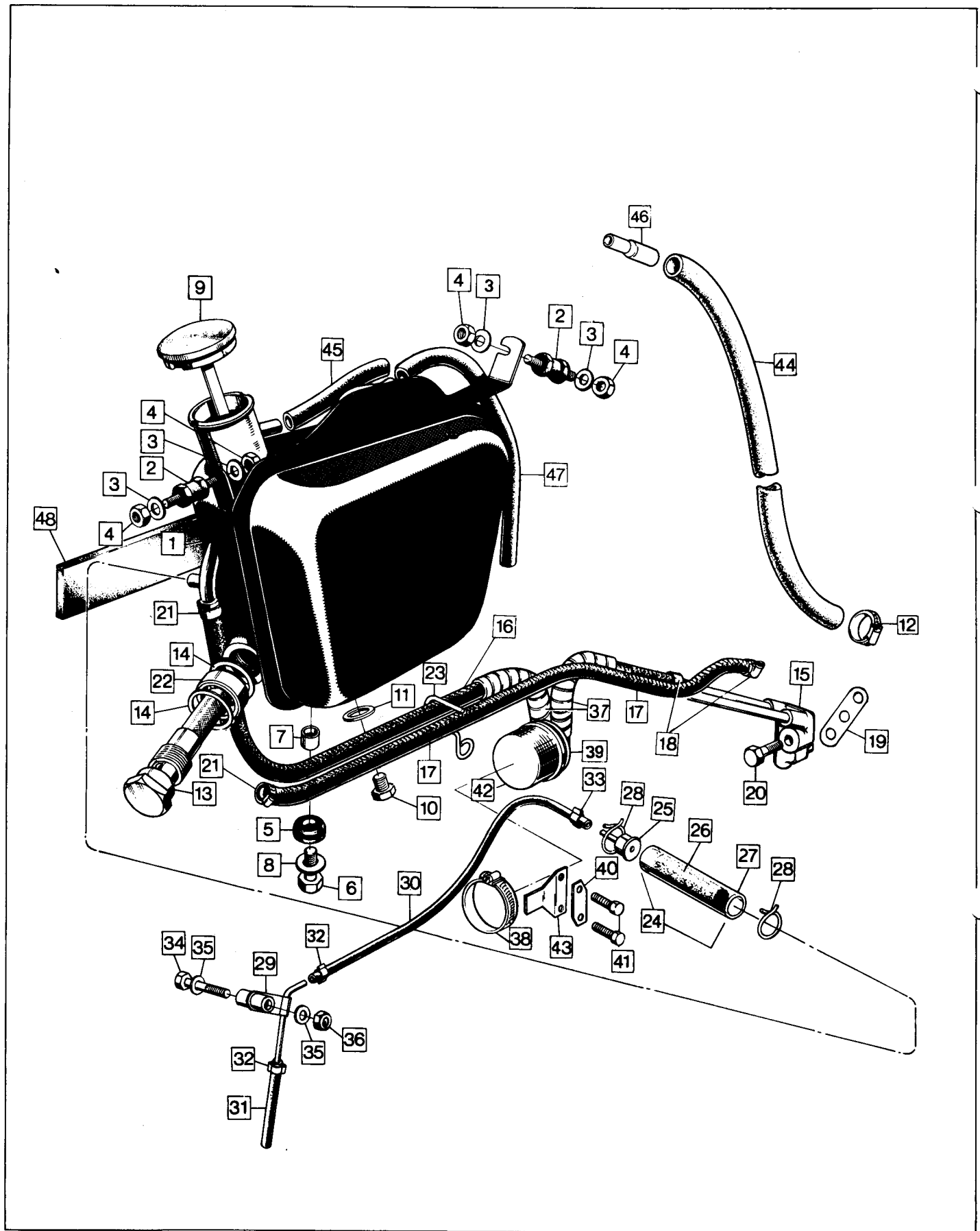
Oil Tank, Oil Pipes, Junction Block, Rear Chain Oiler and Full Flow Oil Filter
