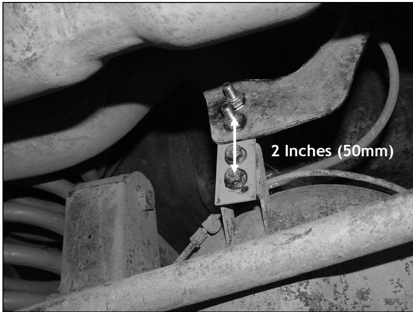
Home made bracket (2" lift), any piece of spare/scrap steel will do.
