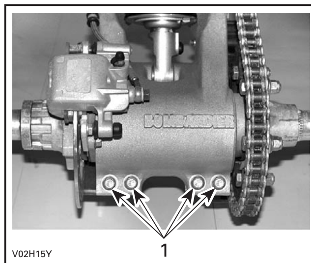
1. Rear axle lock bolts
