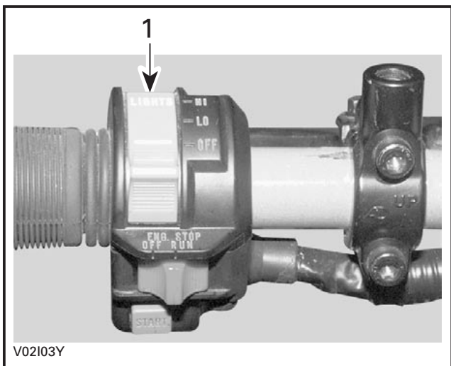
1. Headlamp switch
