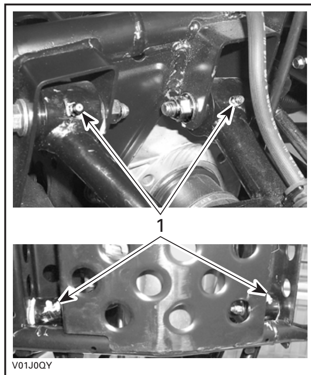
1. Grease fittings
