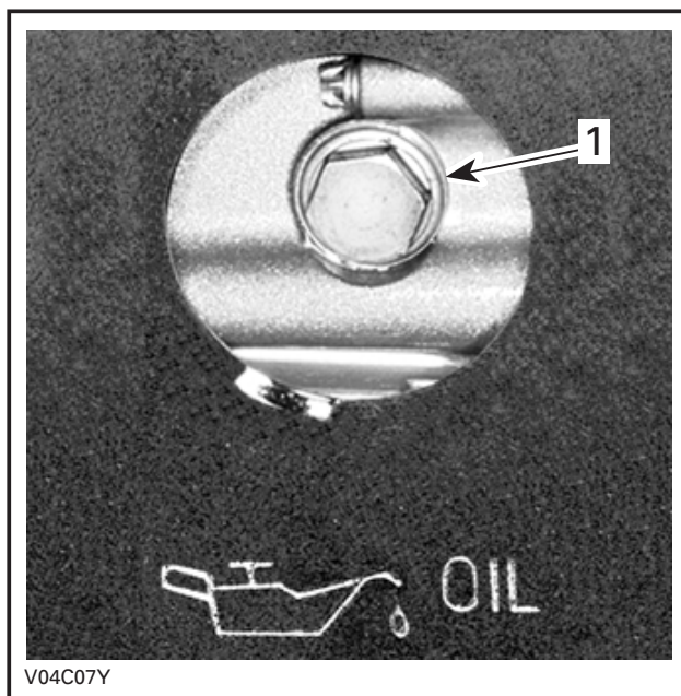
1. Oil drain plug
