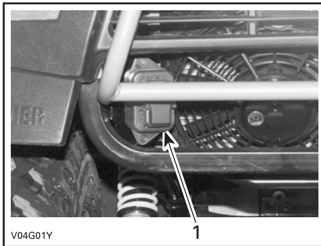
1. Fuse block
