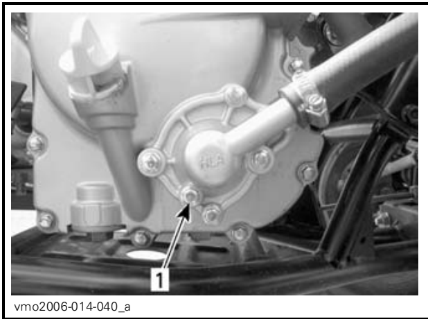
1. Cooling drain plug
