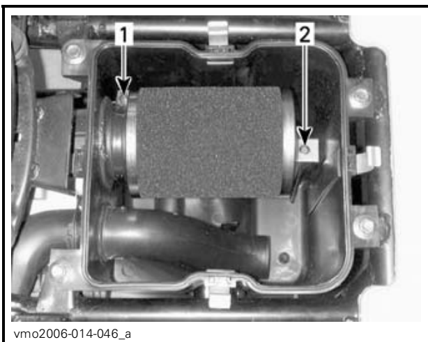
1. Clamp 2. Retaining screw
