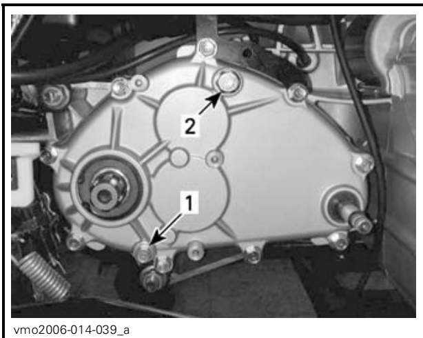
1. Gearbox drain plug 2. Gearbox fill plug
