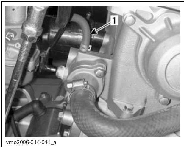
1. By-pass hose
