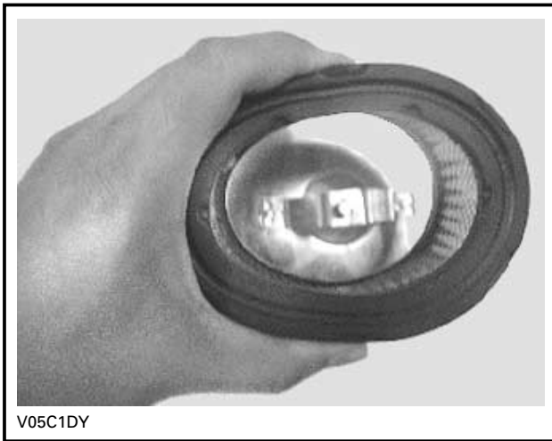
HAND PRESS FILTER INTO AN OVAL SHAPE
