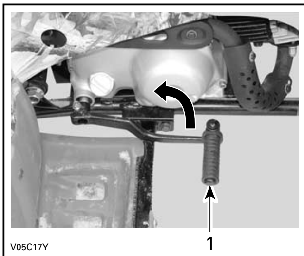
1. Kick start pedal
