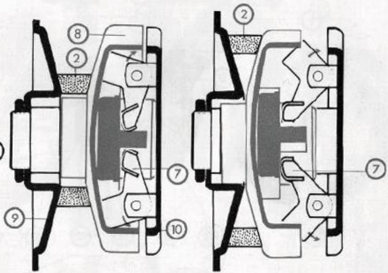
(EXTENSIBLE PULLEY)
