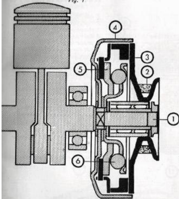
(SINGLE SPEED CLUTCH AND PULLEY)
